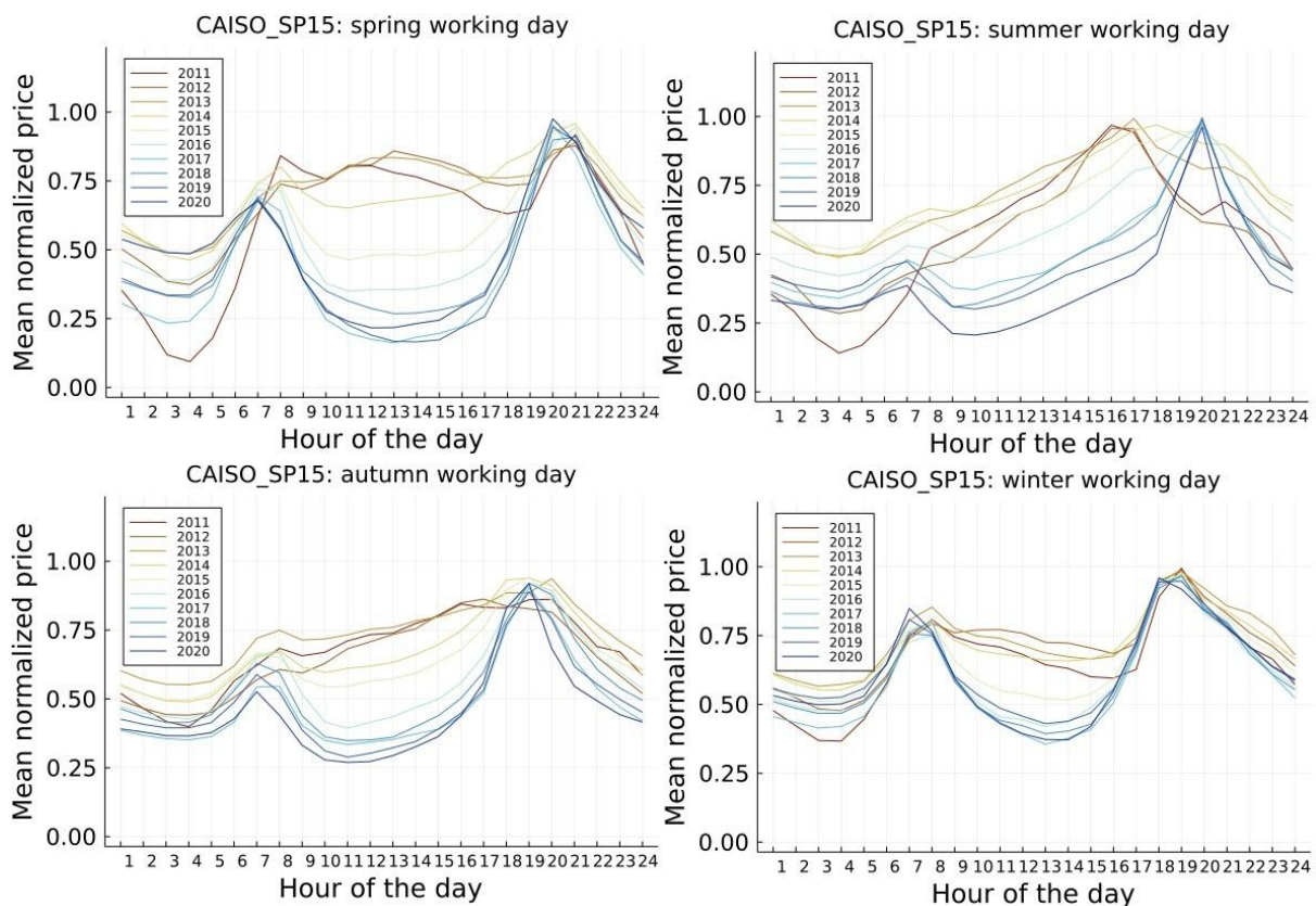
Figure E.1: Average normalized price profiles for working days per season for CAISO SP15 (2011-2020)
